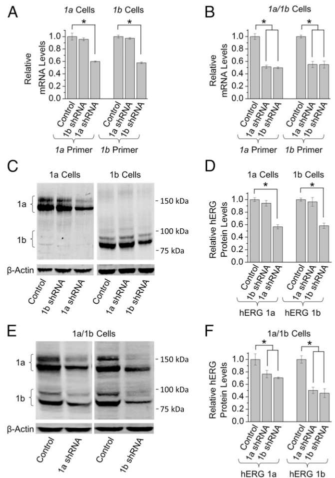
Fig. 1. Cotranslational co-knockdown of hERG 1a and 1b mRNA by transcript-specific shRNA constructs. (A) Effects of transcript-specific shRNA vs. nontargeting control on mRNA levels (mean \pm SEM) in HEK293 cells expressing either hERG 1a (Left) or hERG 1b (Right) (Materials and Methods). (B) Effects of transcript-specific shRNA vs. nontargeting shRNA controls on mRNA levels from HEK293 cells coexpressing hERG 1a and 1b . The mRNA levels were significantly reduced using either shRNA construct. (C) Exemplar and (D) quantification of Western blots corresponding to A showing transcript-specific reduction of hERG 1a (Left) or hERG 1b (Right) protein. (E) Exemplar and (F) quantification of Western blots showing effects of transcript-specific shRNA vs. nontargeting controls on coexpressed hERG 1a and hERG 1b protein. Both subunits were reduced, corresponding to the decrease of mRNA in B ( n = 3-5 ). Statistical significance was assessed using ANOVA and a Bonferroni post hoc t test. *P < 0.05 .
